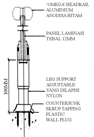
RINCIAN KHUSUS BAGIAN LEG SUPPORT
